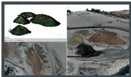
Compute precise surfaces and volume stockpile quantities
